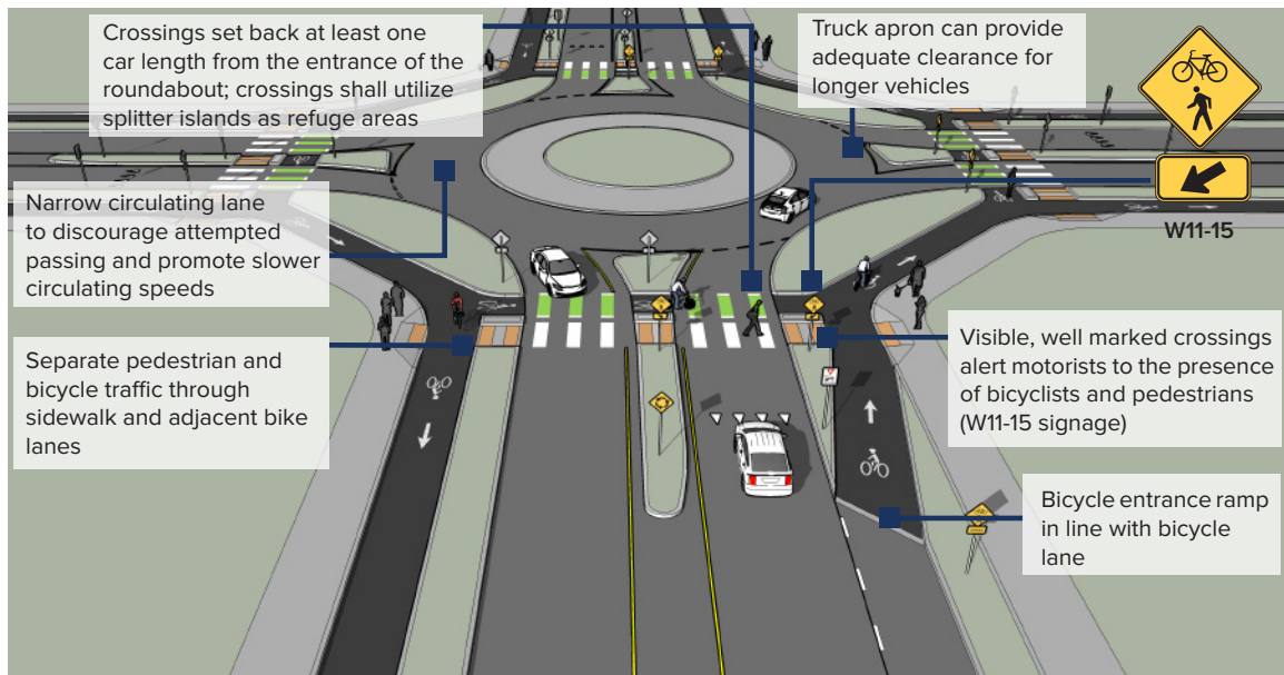
Figure 6.44: Example of Single Lane Roundabout with Bicycle and Pedestrian Crossings & Infrastructure
